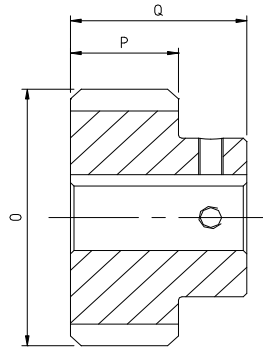
SHAFT PINION
